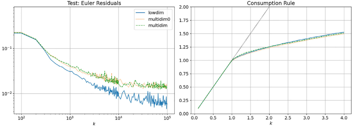
Fig. 9. Multicollinearity and model reduction in the multishock model.
