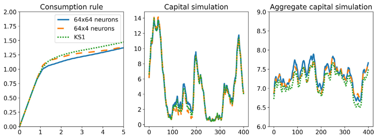
Fig. 14. Comparison of one-moment, 64 \times 64 and 64 \times 4 neuron solutions.
