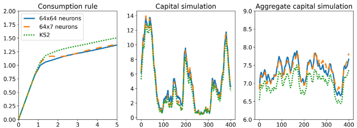
Fig. 15. Comparison of two-moment, 64 \times 64 and 64 \times 7 neuron solutions.
